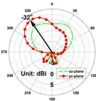
Figure 12: 2D radiation pattern.
