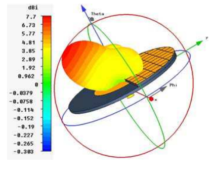
Figure 13: 3D radiation pattern.
